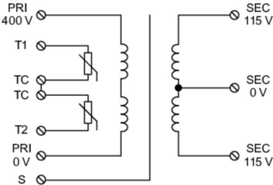
Internal diagram
